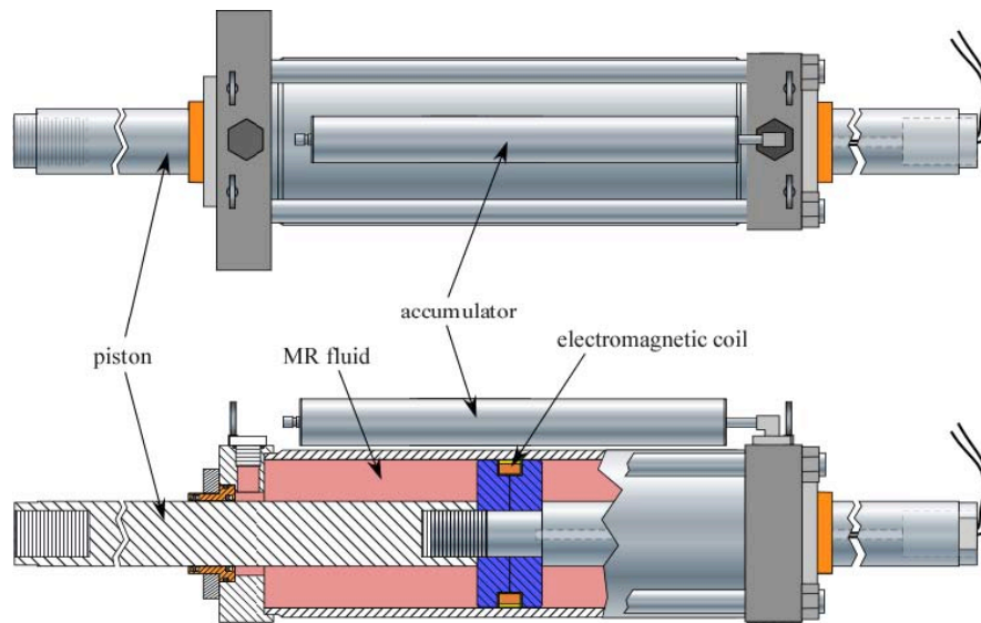
Large-Scale Semiactive Damper Schematic.
